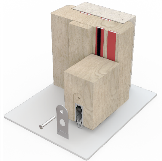
▲ FD60 example: SS seal (Shown with with LP1504 fire seal & LAS8001 si + cladding kit)
