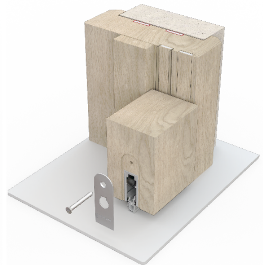
FD60 example: Finesse™ (Shown with LP1504 fire seal & LAS8001 si + cladding kit)
