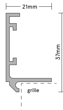
↑ LV2221 ALUMINIUM FLANGE
