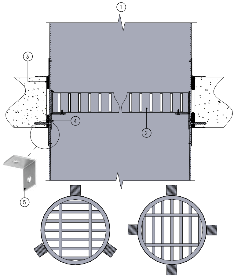
FIXING OPTION 1
